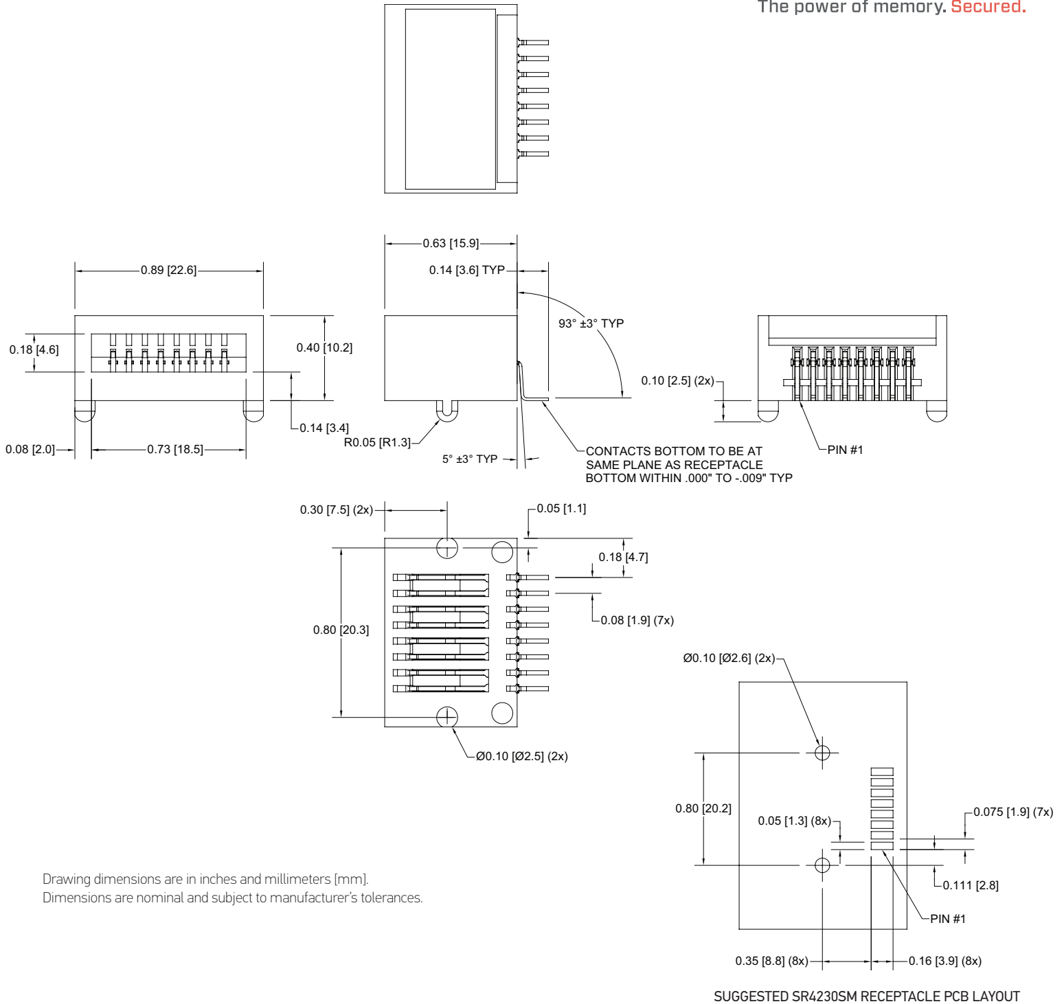
SUGGESTED SR4230SM RECEPTACLE PCB LAYOUT
